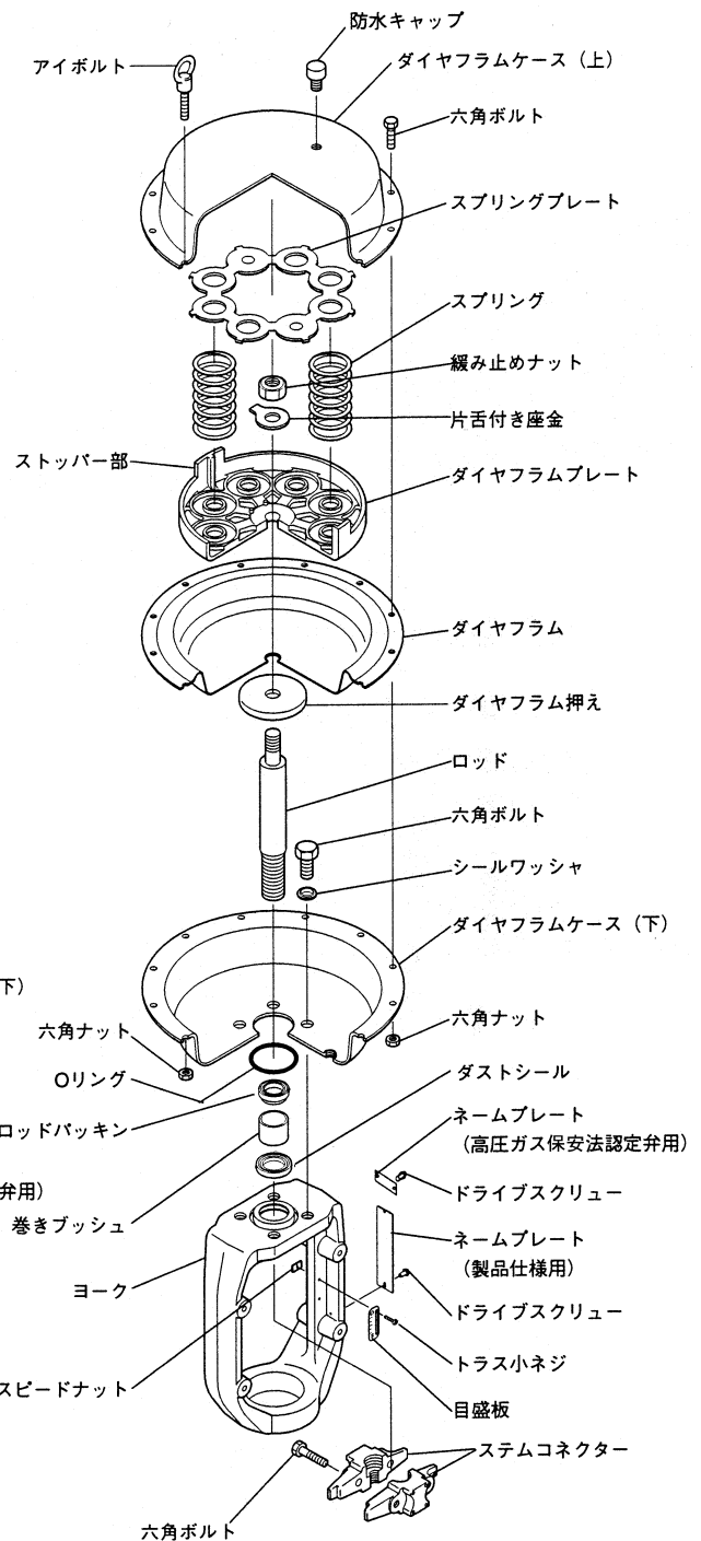
図6-4 PSA3R, PSA4R
