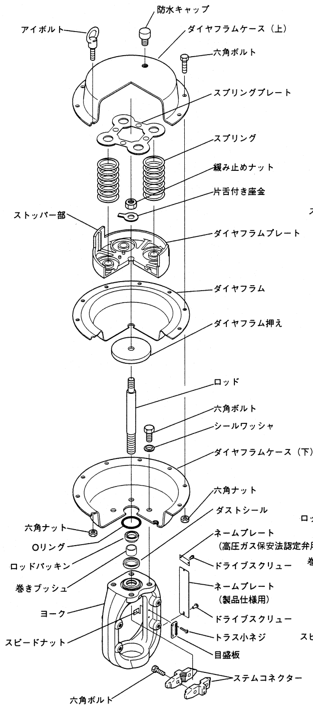
図6-3 PSA1R, PSA2R
